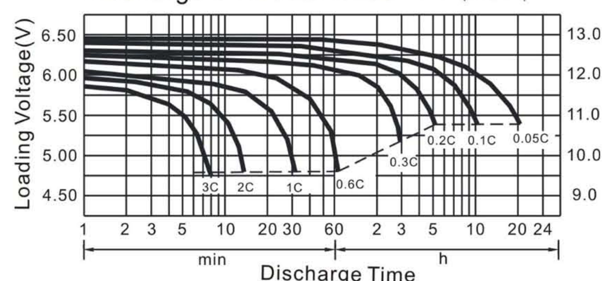
Discharge Characteristics 77°F (25°C)
